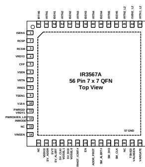
Figure 2: IR3567A Package Top View
