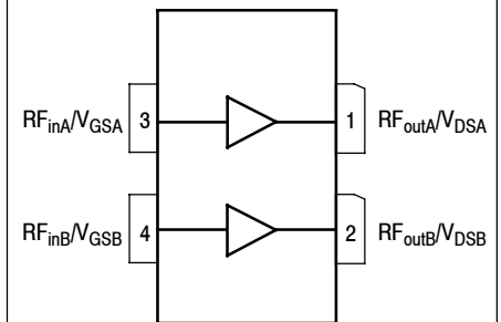
Figure 1. Pin Connections
