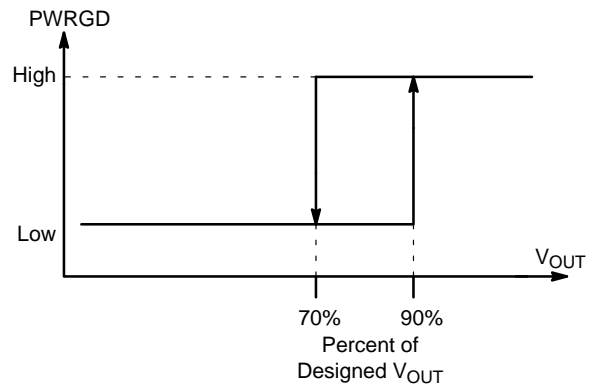
Figure 23. PWRGD Assertion
