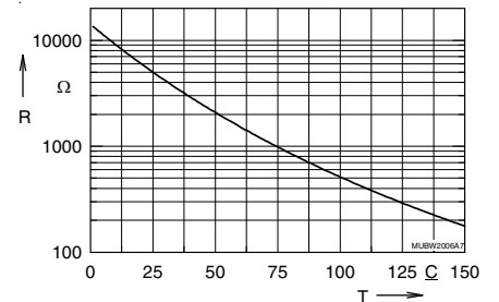
Typ. thermistor resistance versus temperature
