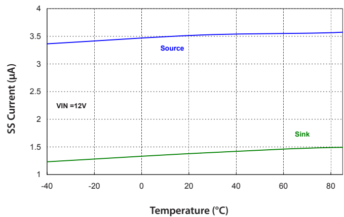
SS Current vs. Temperature
