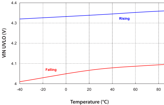
UVLO Threshold vs. Temperature
