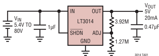
5V Supply with Shutdown
